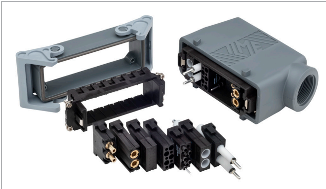
Multipole connectors for voltages up to 10,000 V and currents up to 30 A.
